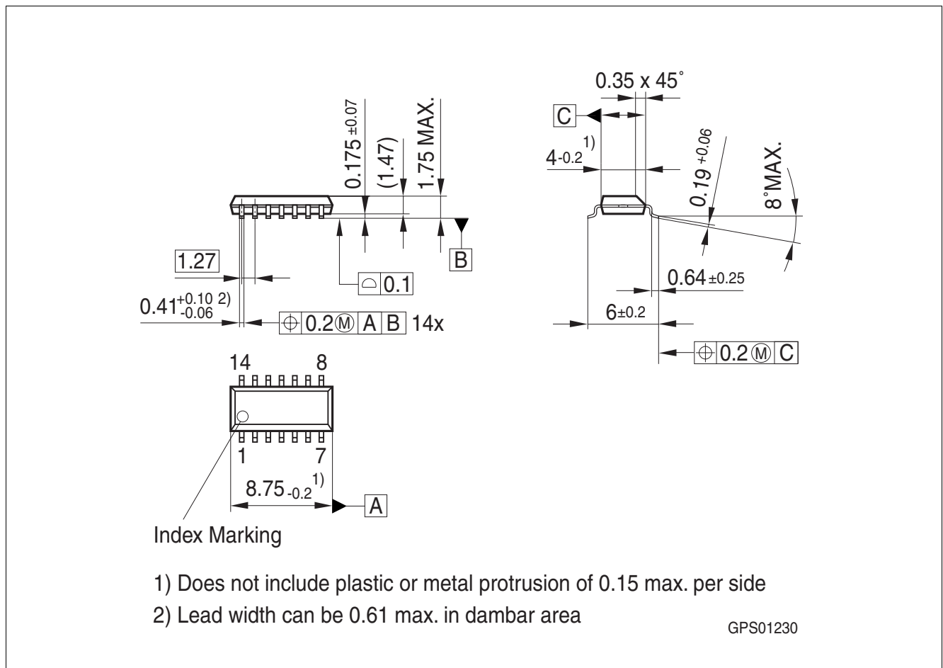
Figure 13 Outline PG-DSO-14
