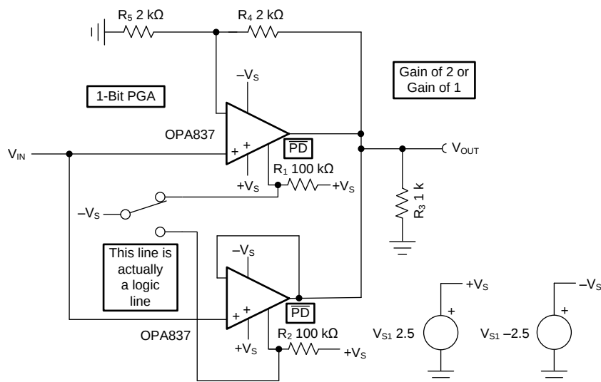
Figure 88. 1-Bit PGA
