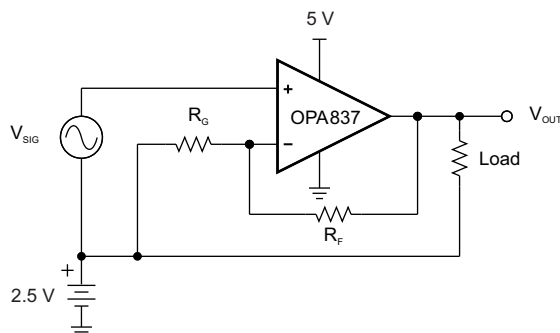
Figure 69. Single-Supply Concept
