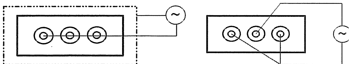
Fig.4 Measurement of Insulation resistance and Withstand voltage
