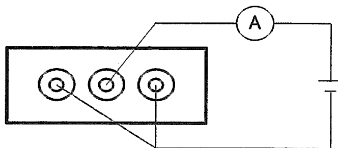
Fig.5 Measuring leak current between the adjacent contacts
