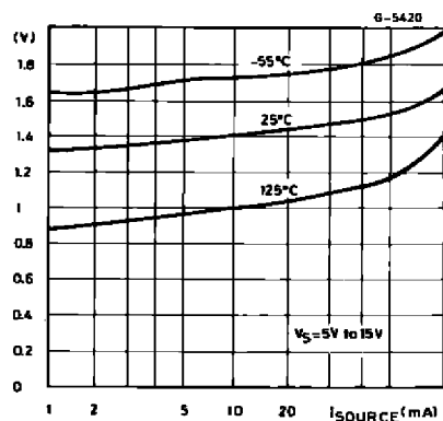
Figure 7 : High Output Voltage Drop versus Output
