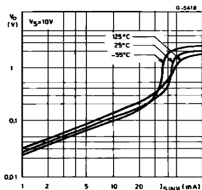
Figure 5 : Low Output Voltage versus Output Sink Current
