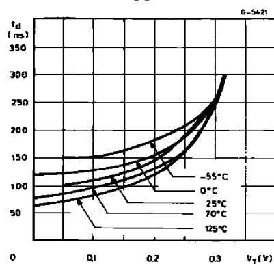
Figure 9 : Propagation Delay versus Voltage Level of Trigger Value
