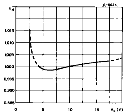
Figure 9 : Propagation Delay versus Voltage Level of Trigger Value
