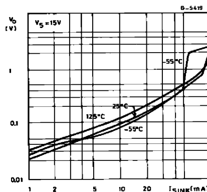
Figure 6 : Low Output Voltage versus Output Sink Current
