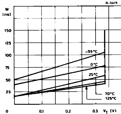
Figure 1 : Minimum Pulse Width Required for Trigering
