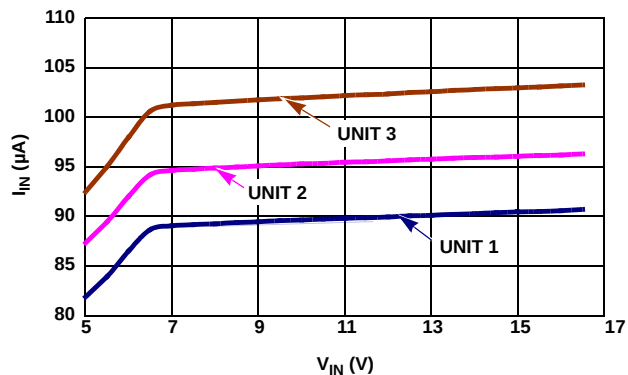
FIGURE 30. I_{IN} vs V_{IN} , 3 UNITS
