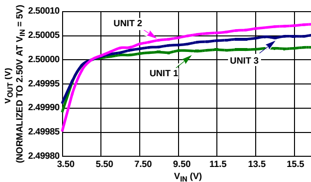
FIGURE 18. LINE REGULATION
