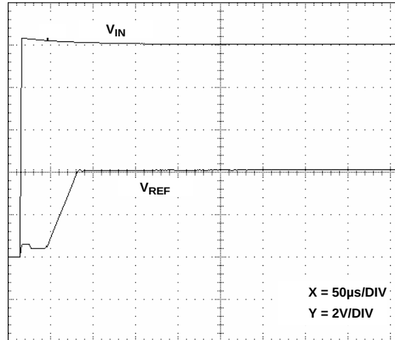
FIGURE 39. TURN-ON TIME
