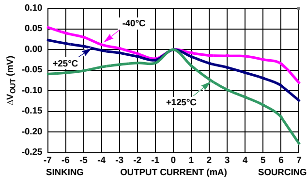
FIGURE 48. LOAD REGULATION
