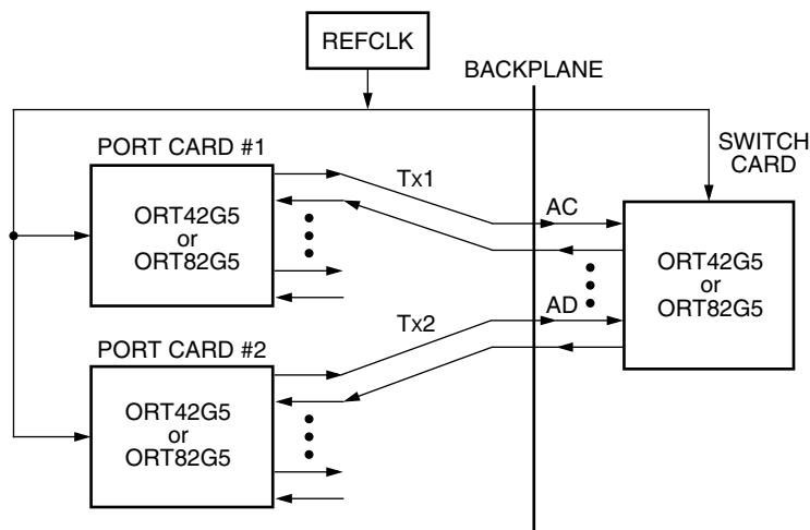
Figure 38. Distributed Reference Clock to Rx And Tx Devices
