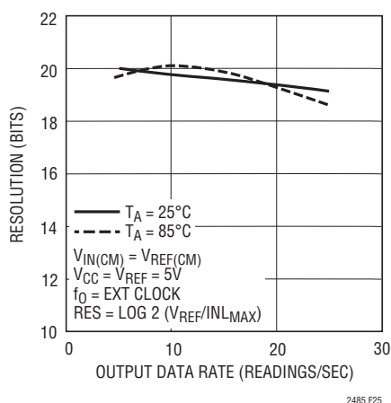
Figure 25. Resolution ( \text{INL}_{MAX} \leq 1\text{LSB} ) vs Output Data Rate and Temperature
