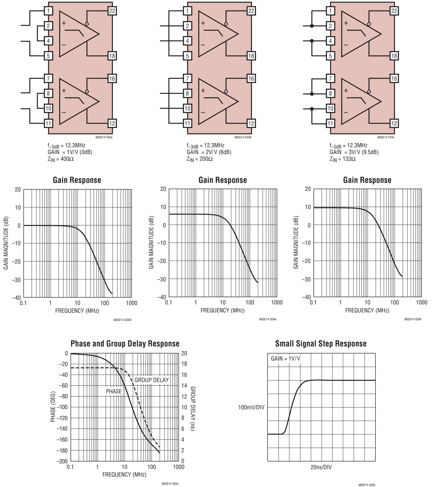
Figure 4. f_{-3dB} = 12.3\text{MHz} Filter Configurations without External Components
