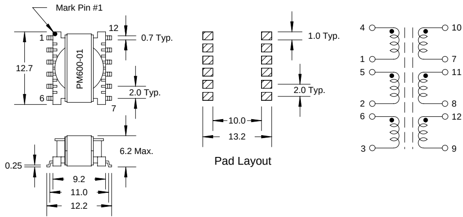
PM600-xx
