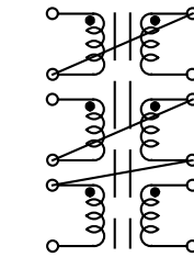
Figure 9 Turns ratio: 2:3 or 3:2
