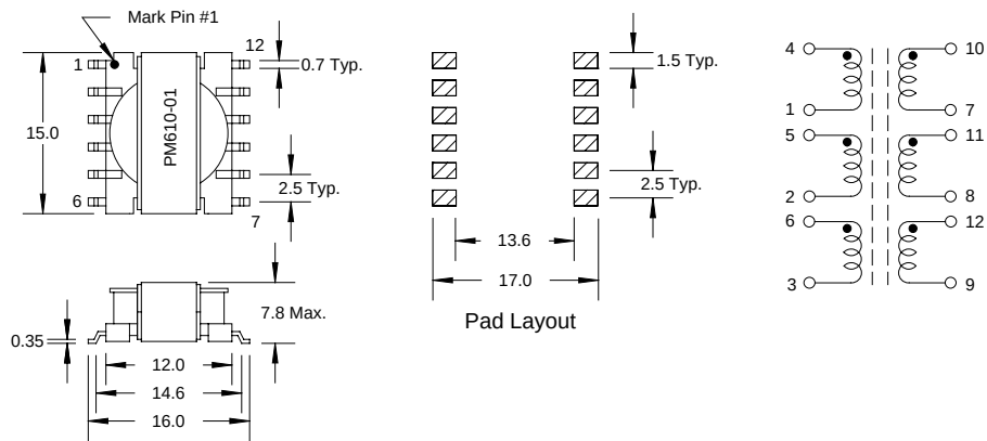
PM610-xx
