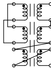
Figure 4 Turns ratio: 1:4 or 4:1
