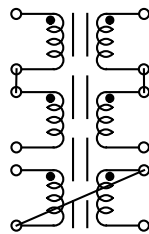
Figure 2 Turns ratio: 1:1:1
