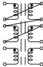
Figure 7 Turns ratio: 4:1:1
