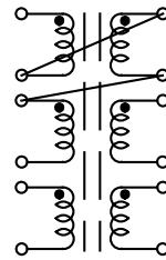
Figure 8 Turns ratio: 3:1:1:1
