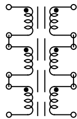
Figure 2 Turns ratio: 1:1
