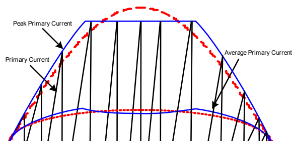
Figure 6: Primary Current Waveform of Flyback PFC with the MP44011
