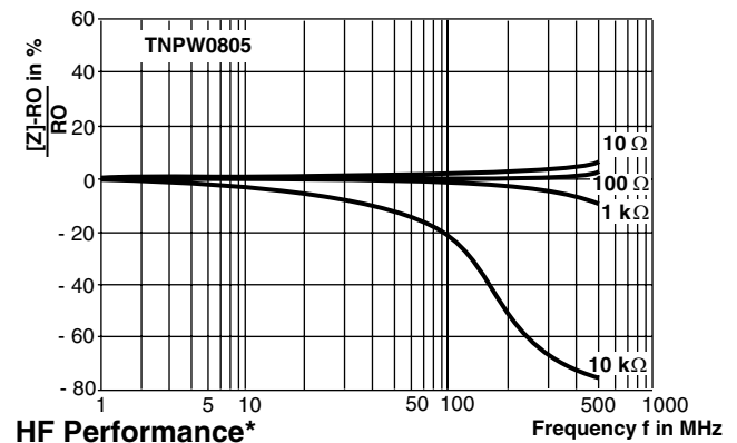
HF Performance*
