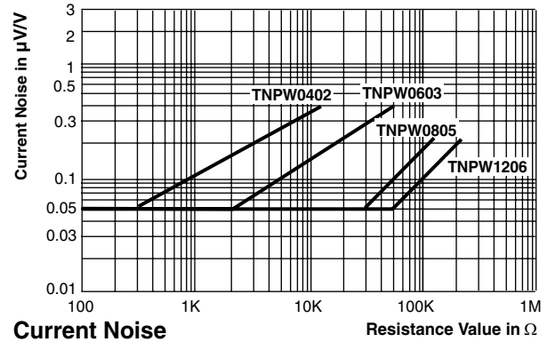
Current Noise
