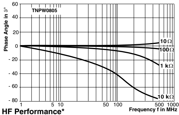
HF Performance*
