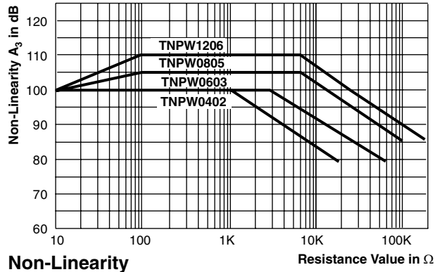
Non-Linearity
