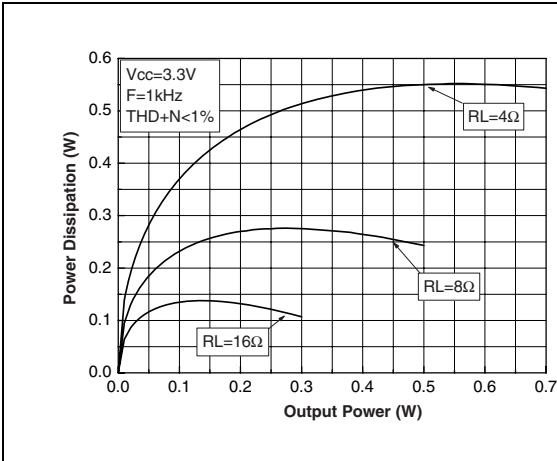
Figure 32. Power dissipation vs. P_{out}
