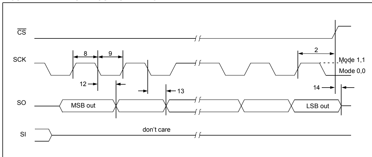
FIGURE 11-11: SPI™ OUTPUT TIMING
