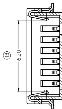
SECTION Z-Z
