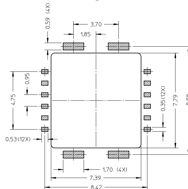
RECOMMENDED PCB LAYOUT TOLERANCE:0.05mm
