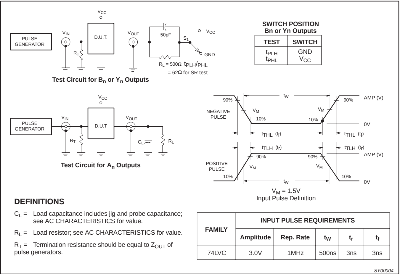
Waveform 5.
