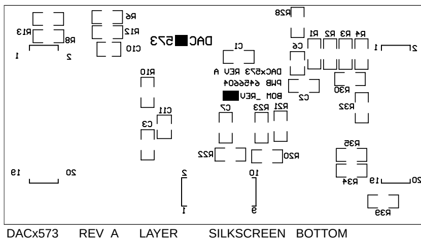
Figure 2-6. Bottom Silkscreen
