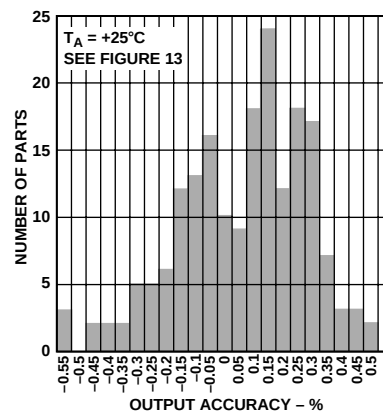
Figure 12. Output Accuracy Distribution, V_{OUT} = 2.0\text{ V}
