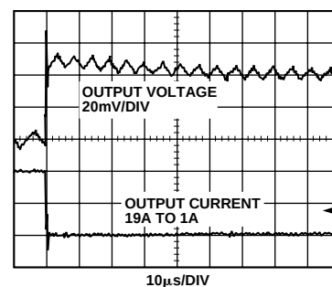
Figure 9. Transient Response, 19 A-1 A of Figure 2 Circuit
