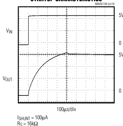
MAX6138_50 STARTUP CHARACTERISTICS
