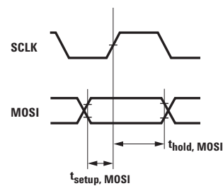
Figure 13. MOSI setup
