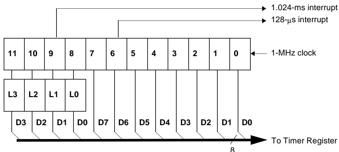
Figure 12-3. Timer Block Diagram
