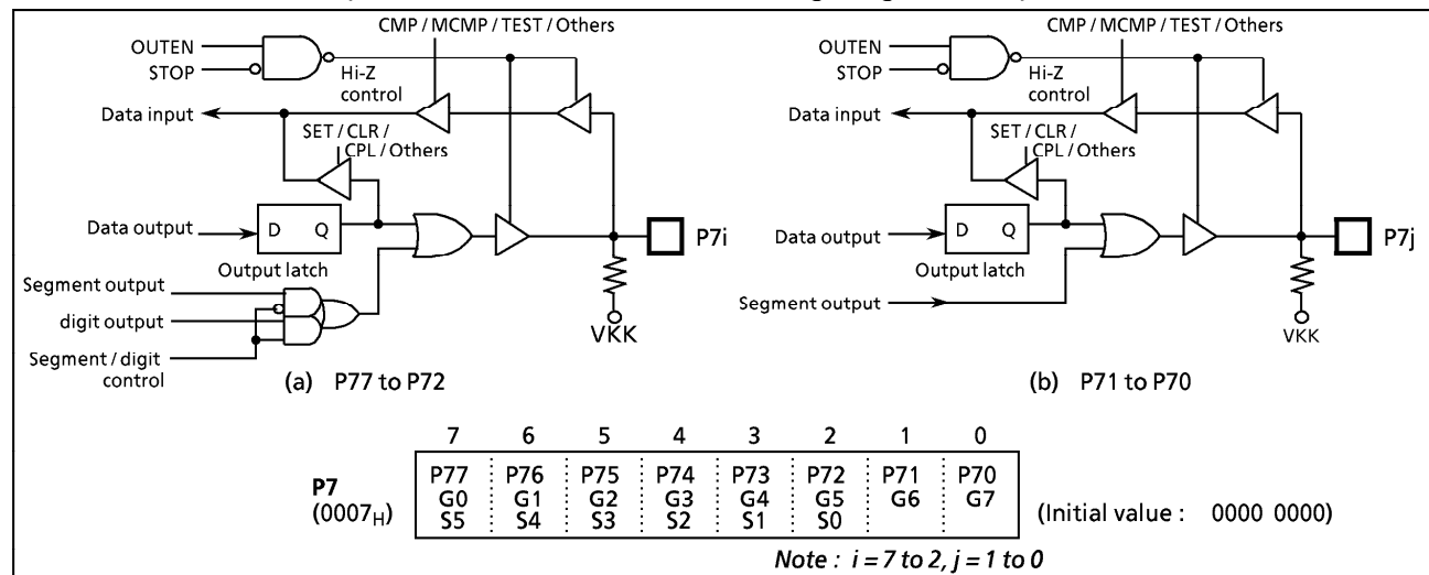
Figure 2-10. Port P7
