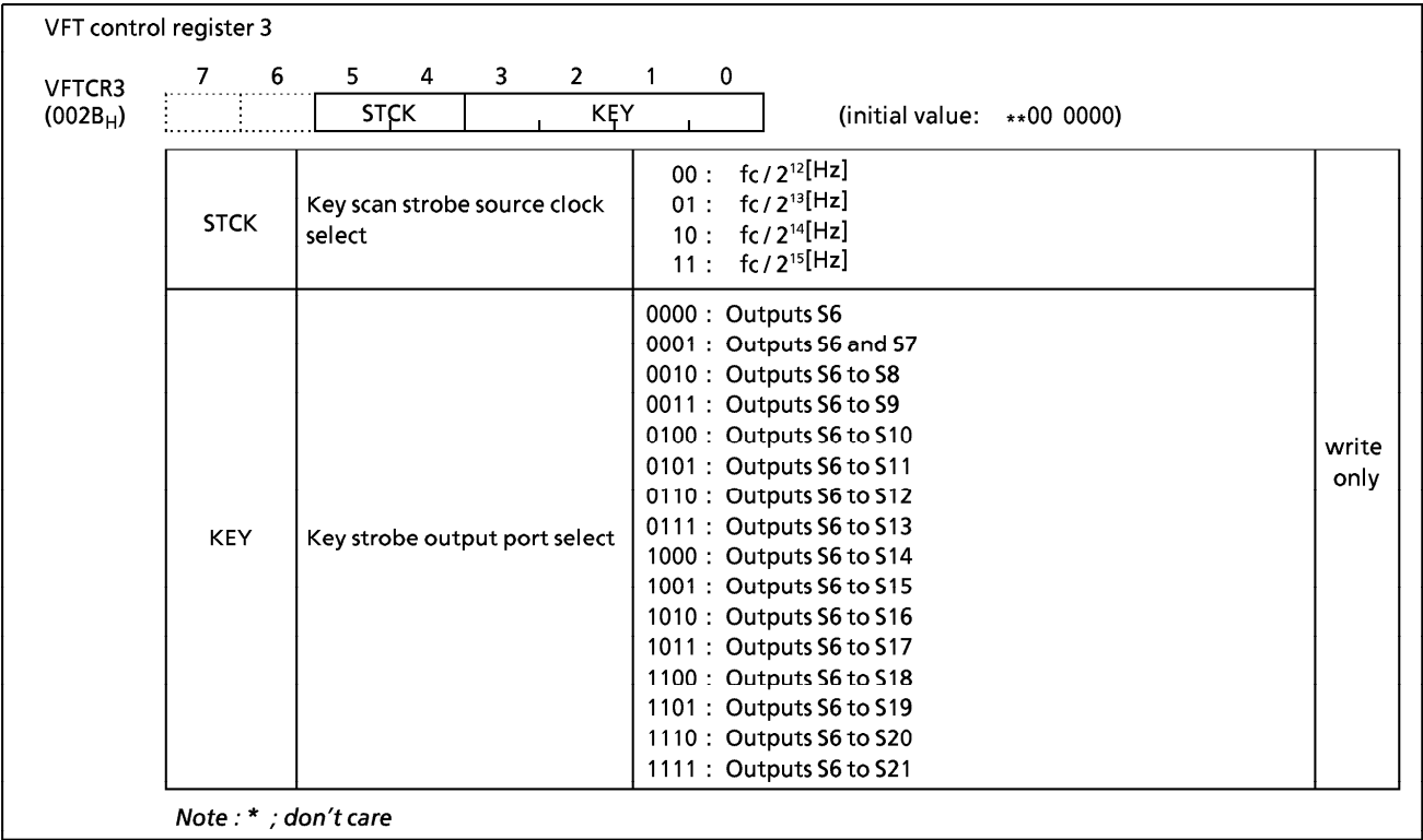
Figure 2-52. (b) VFT Control Register 3
