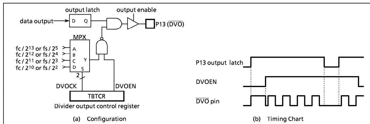
Figure 2-17. Divider Output
