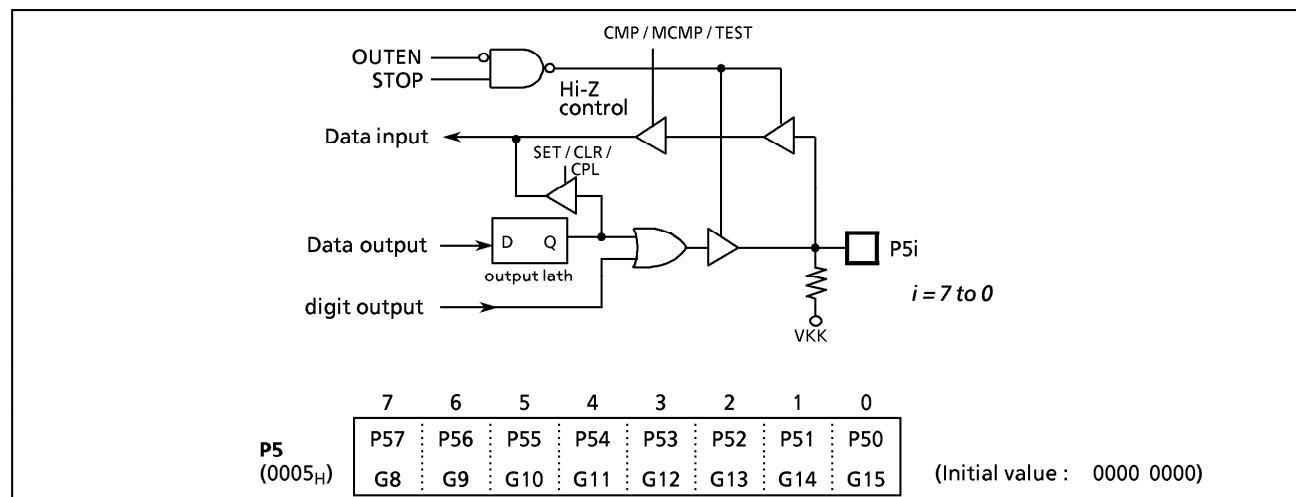
Figure 2-8. P5 Port
