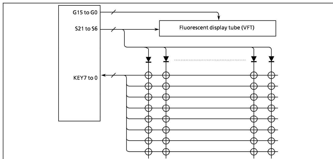
Figure 2-59. Key Matrix Configuration Example
