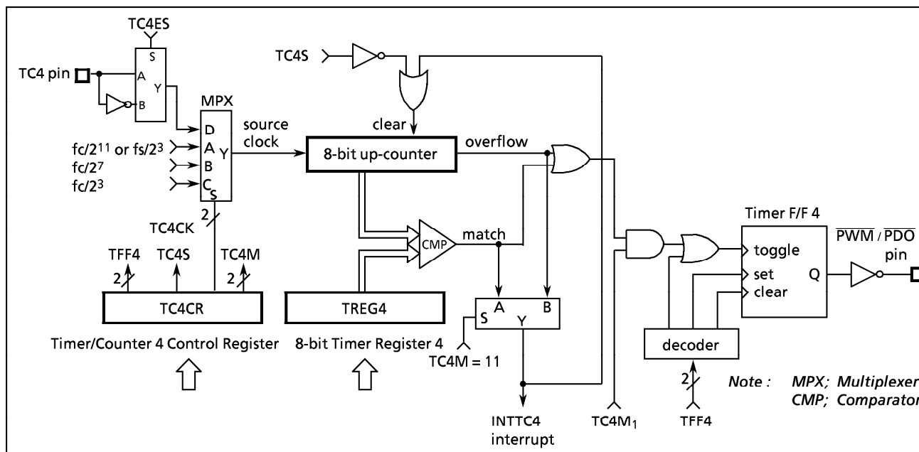
Figure 2-33. Timer/Counter 4
