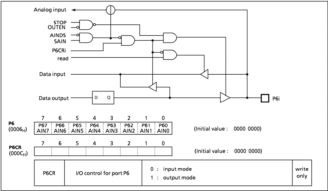
Figure 2-9. Port P6
