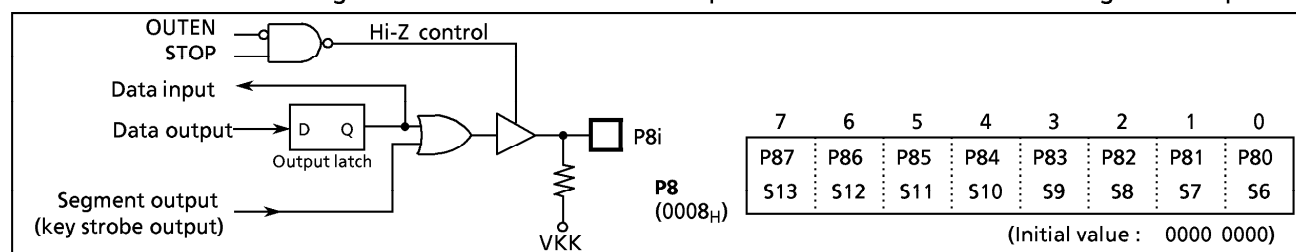
Figure 2-11. Port P8
