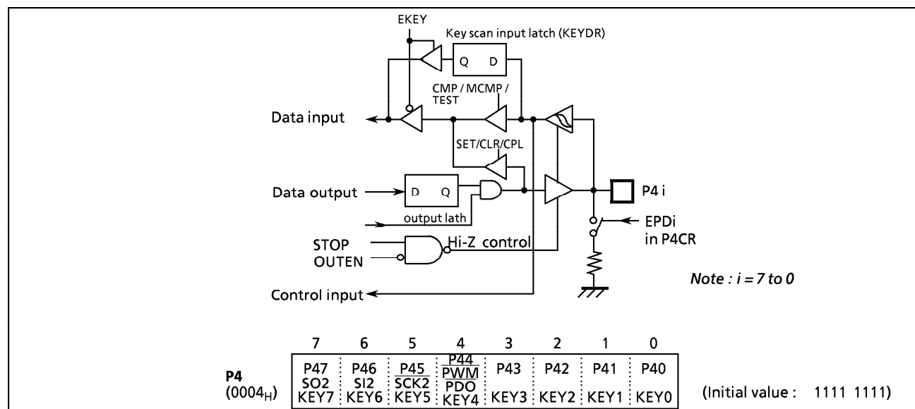
Figure 2-7. Port P4
