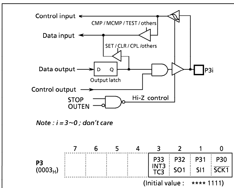
Figure 2-6. Port P3
