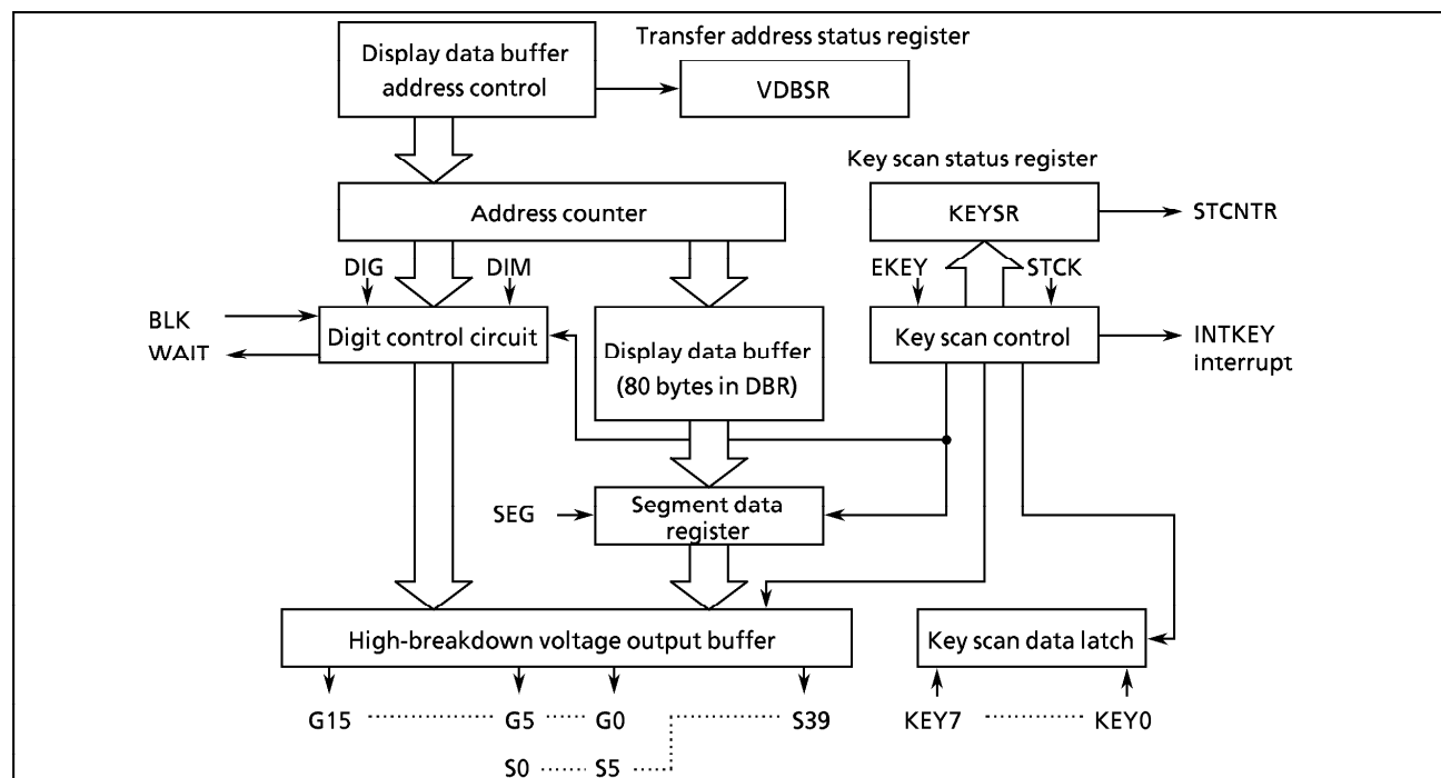
Figure 2-51. VFT
