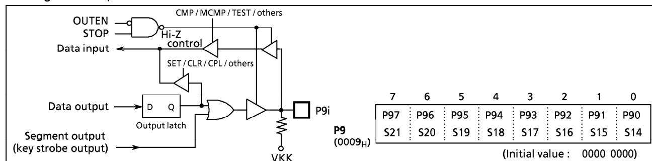
Figure 2-12. Port P9
