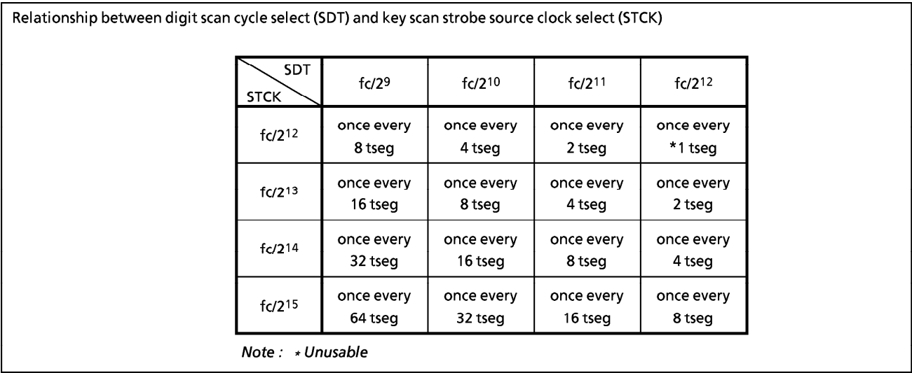
Figure 2-53. Relationship between Digit Cycle Select and Key Scan Strobe Source Clock Select
