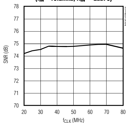
SNR vs. SAMPLING FREQUENCY ( f_{IN} = 15.2MHz , A_{IN} = -2dBFS )
