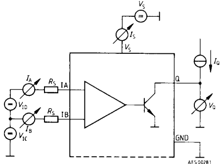
Test Circuit 2
