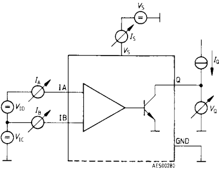
Test Circuit 1
