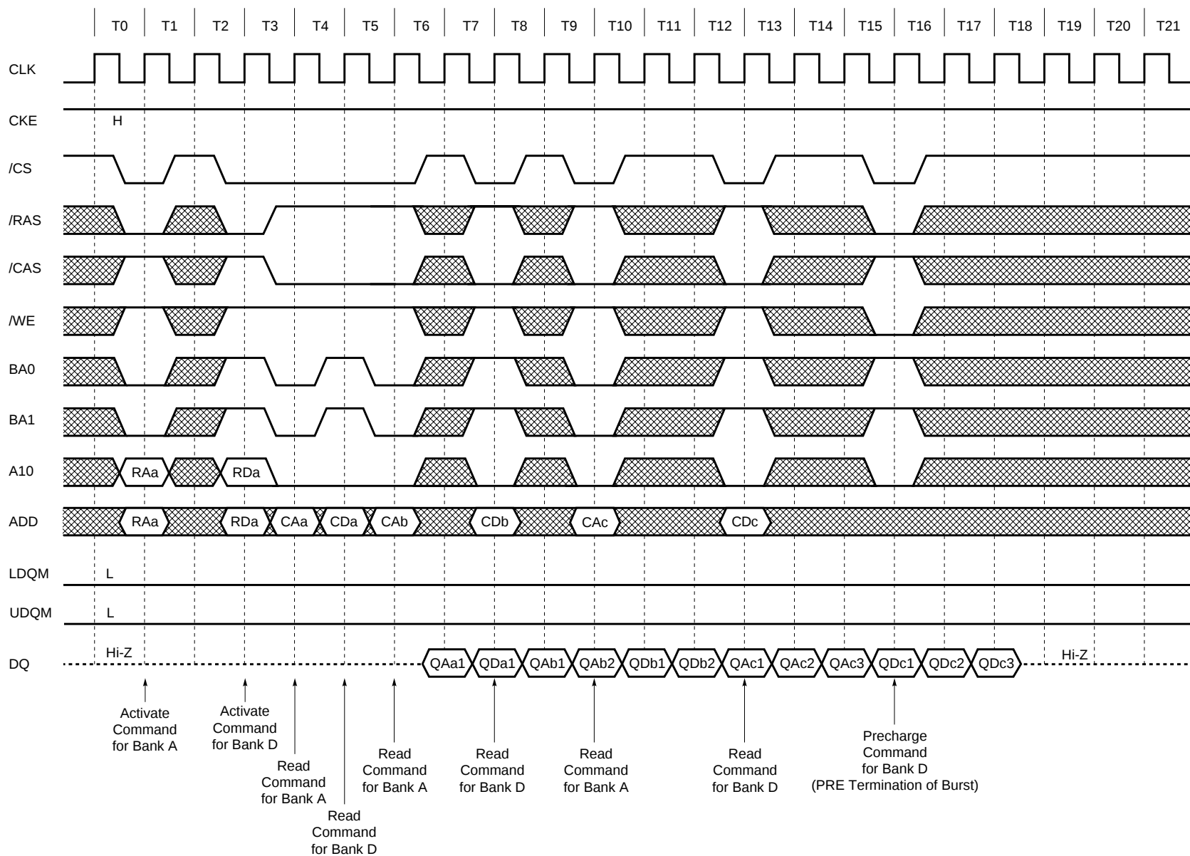
Full Page Random Column Read (Burst Length = Full Page, /CAS Latency = 3)
