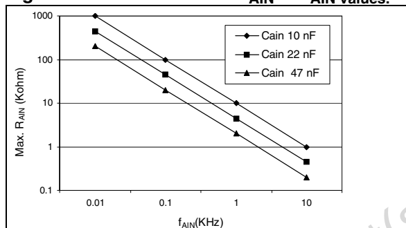
Figure 92. Recommended C_{AIN} & R_{AIN} values. 2)
