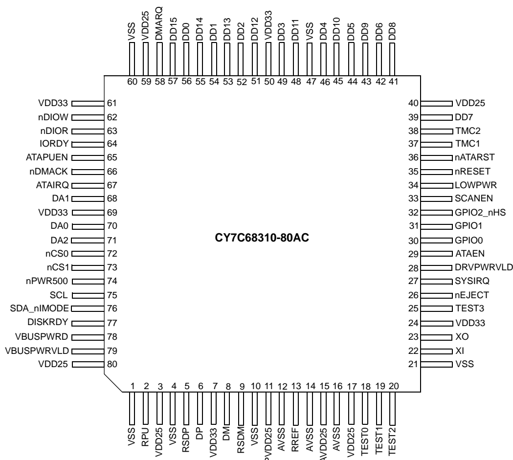
Figure 4-1. 80-pin TQFP
