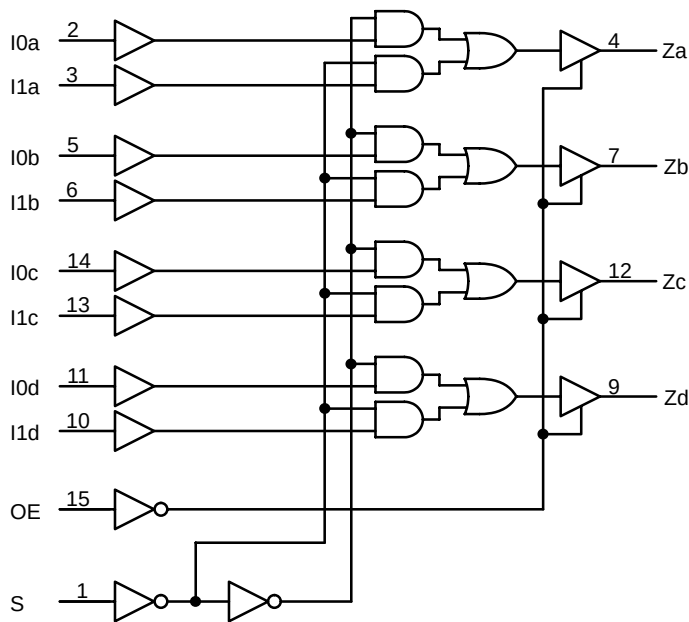
Figure 2. Logic Diagram
