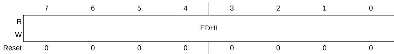
Figure 4-15. EEPROM Data High Register (EDATAHI)
