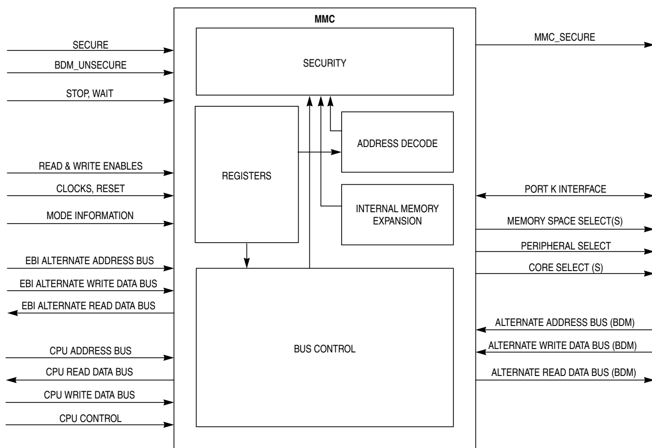
Figure 20-1. MMC Block Diagram
