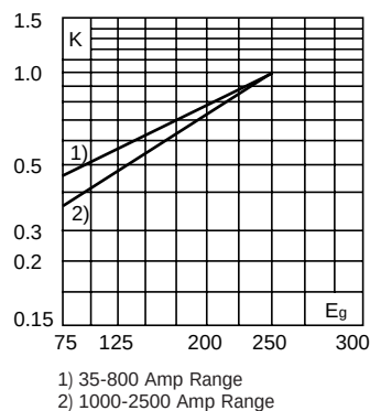
Fig. 1: 35-800 Amp Range
