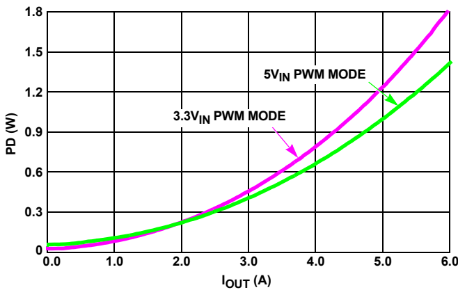
FIGURE 9. POWER DISSIPATION vs LOAD (1MHz, V_{OUT} = 1.8\text{V} )
