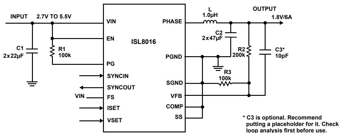
FIGURE 2. TYPICAL APPLICATION DIAGRAM - SINGLE CHIP 6A
