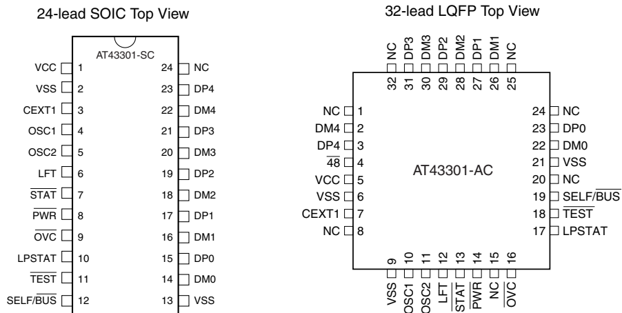
Figure 1-1. Pin Configurations
