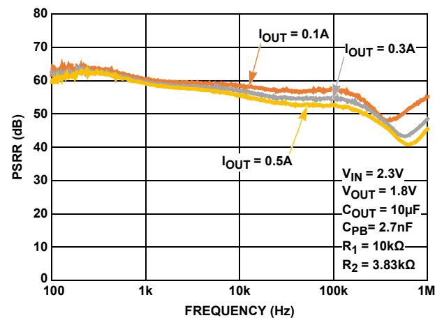
FIGURE 2. PSRR
