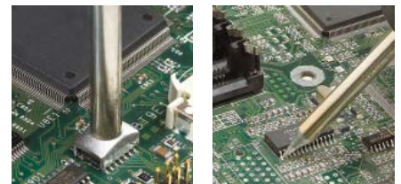
MFR-2200 Series Hand-pieces A. MFR-H4-TW Precision Tweezers B. MFR-H2-ST Soldering Tip C. MFR-H1-SC Soldering Cartridge
