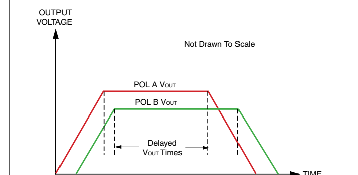
Figure 13. Staggered or Sequential Phasing—Exclusive (Fixed Cascaded Delays)
