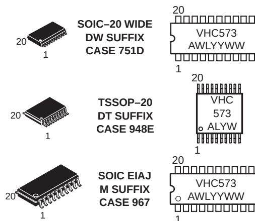
MARKING DIAGRAMS
