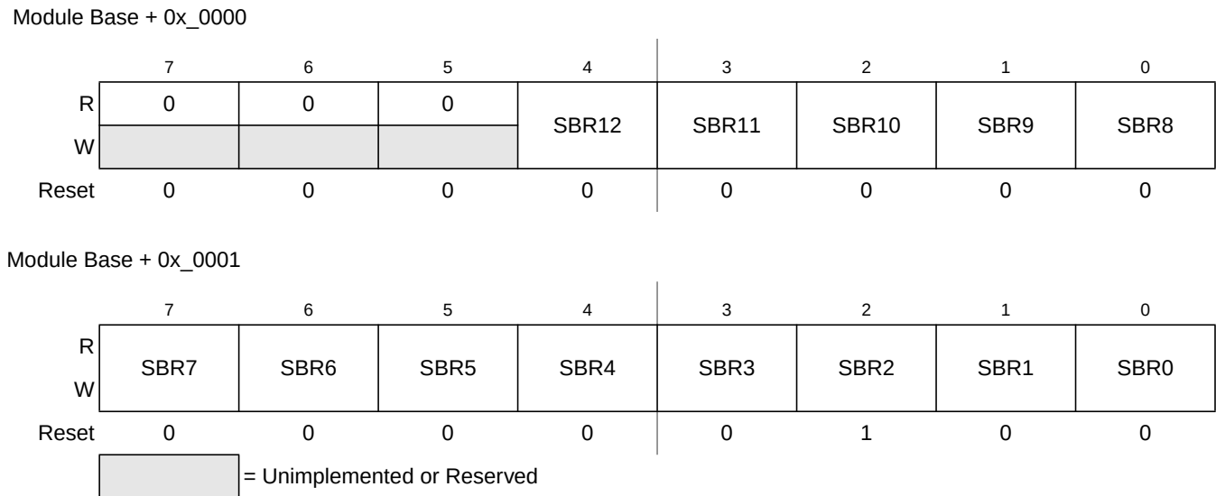
Figure 11-3. SCI Baud Rate Registers (SCIBDH and SCIBDL)
