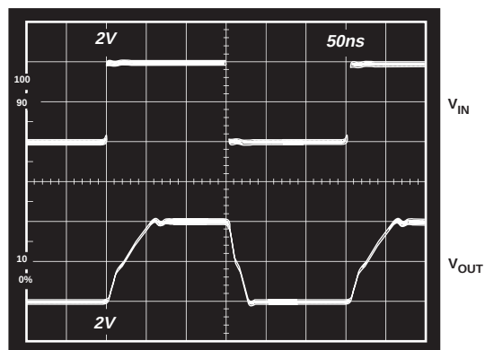
Figure 23. Large Signal Pulse Response, Gain = +1, ( R_F = 750\ \Omega , R_L = 150\ \Omega , V_S = \pm 5\text{ V} )
