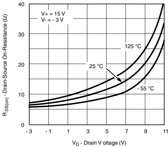
R_{\text{DS(on)}} vs. Drain Voltage DG641, DG643
