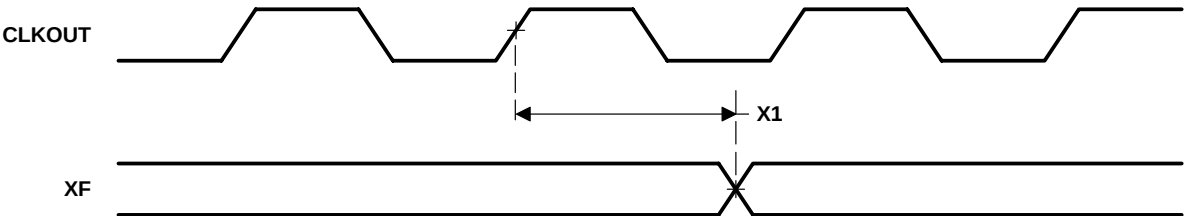
Figure 5–17. XF Timing
