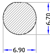
PANEL CUTOUT
