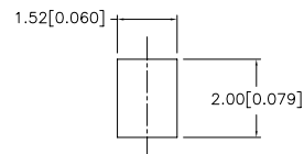
VIEW C SCALE: 4/1 1X FOR 2 PORT 3X FOR 4 PORT
