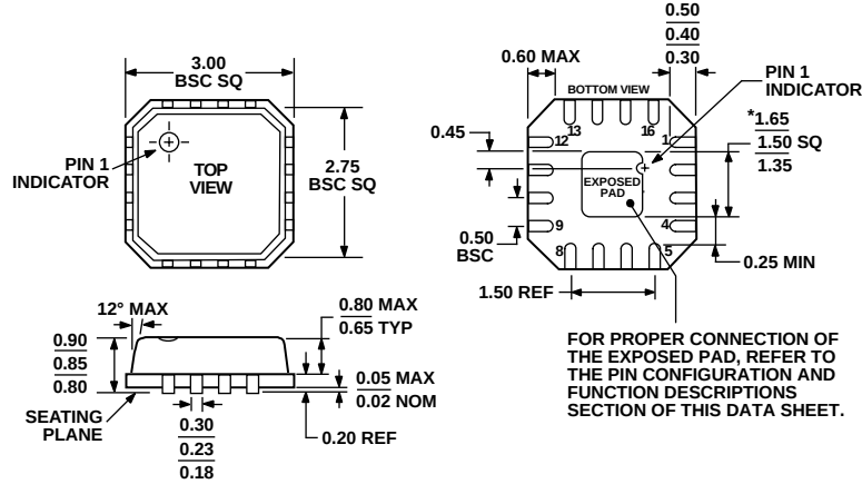
Figure 54. 16-Lead Lead Frame Chip Scale Package [LFCSP_VQ] 3 mm × 3 mm Body, Very Thin Quad (CP-16-3) Dimensions shown in millimeters
