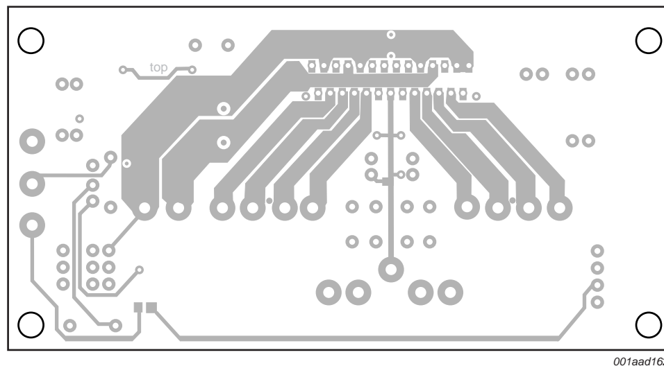
Fig 33. PCB layout of test and application circuit; copper layer top
