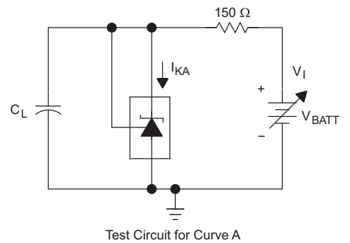
Test Circuit for Curve A
