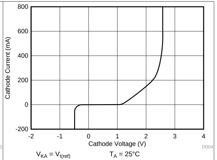
Figure 4. Cathode Current vs Cathode Voltage
