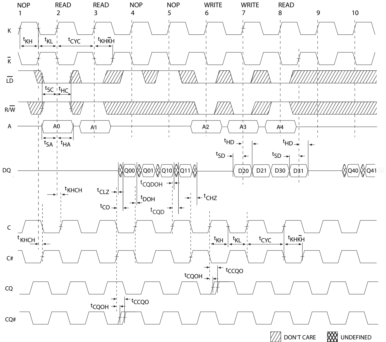
Figure 5. Read/Write/Deselect Sequence [26, 27, 28]
