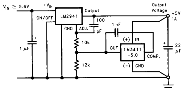
FIGURE 7. Precision 5V 1A Low Dropout Regulator
