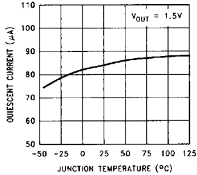
Quiescent Current
