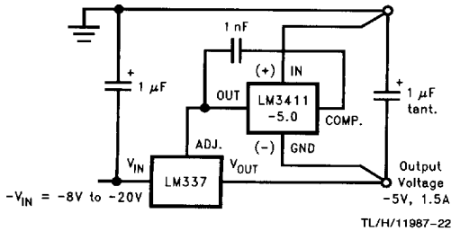
FIGURE 10. Precision Negative Voltage Regulator
