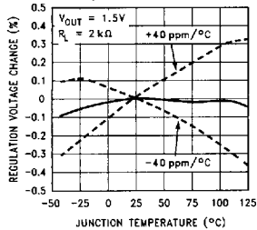
Normalized Temperature Drift
