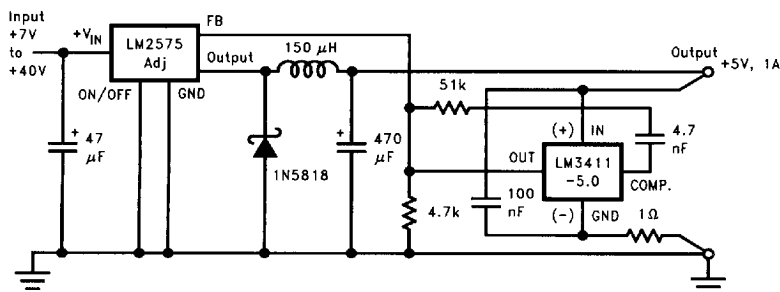
FIGURE 5. Precision 1A Buck Regulator
