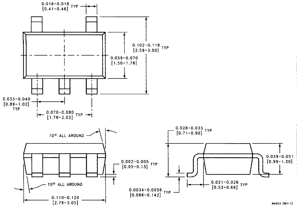
5-Lead Small Outline Package (M5) Order Number LM3411M5-3.3, LM3411AM5-3.3, LM3411M5-5.0 or LM3411AM5-5.0 NS Package Number MA05A
