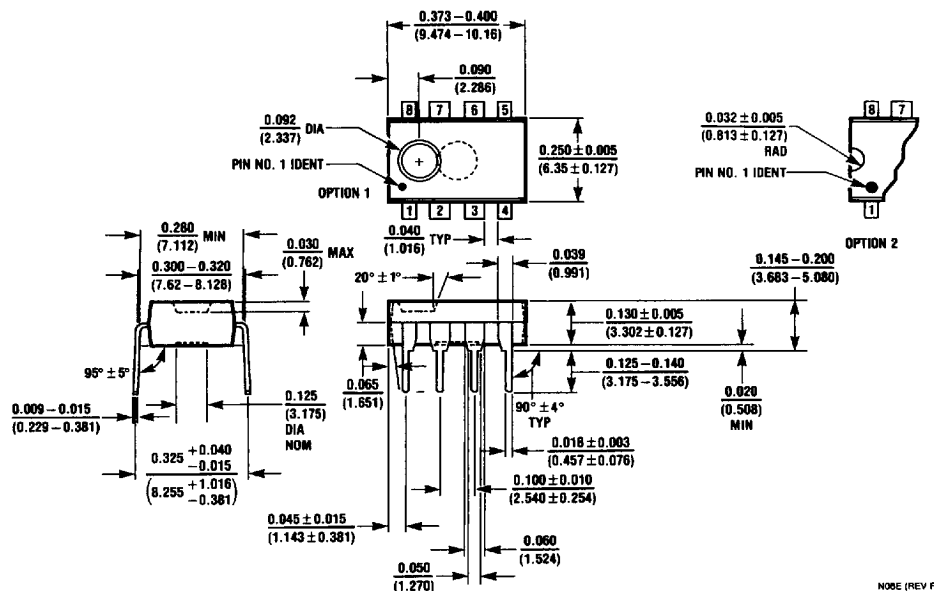
8-Lead Dual-In-Line Package (N) Order Number LM3411N-3.3, LM3411AN-3.3, L3411N-5.0 or LM3411AN-5.0 NS Package Number N08E
