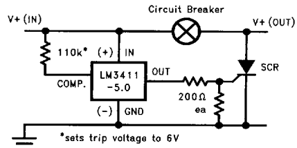
FIGURE 16. Overvoltage Crowbar
