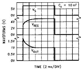
Response Time for 5V Version ( C_c = 10nF )
