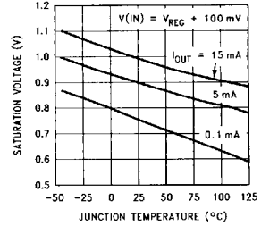
Output Saturation Voltage (V) SAT
