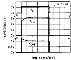
Response Time for 3.3V Version ( C_c = 10nF )
