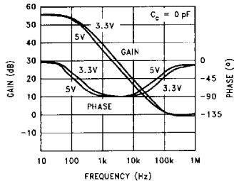
Bode Plot
