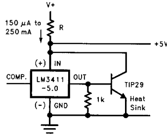
FIGURE 14. 250 mA Shunt Regulator
