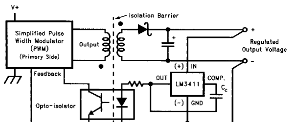
Basic Isolated DC/DC Converter
