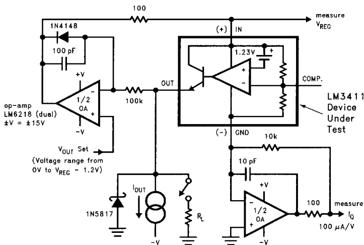
FIGURE 2. LM3411 Test Circuit
