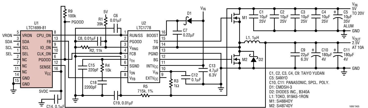
SMBus Controlled High Efficiency DC/DC Converter
