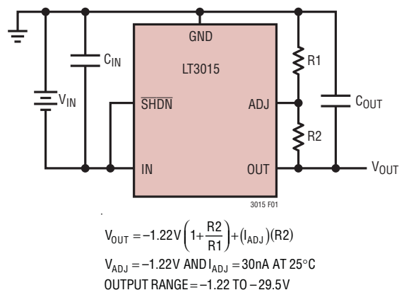
Figure 1. Adjustable Operation
