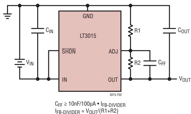
Figure 2. Feedforward Capacitor for Fast Transient Response, Low Noise, and High PSRR
