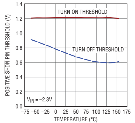
Positive SHDN Pin Thresholds
