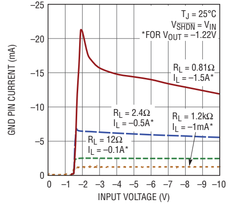
LT3015 GND Pin Current
