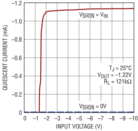
LT3015 Quiescent Current
