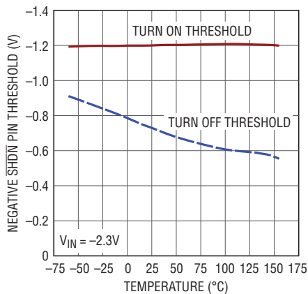
Negative SHDN Pin Thresholds
