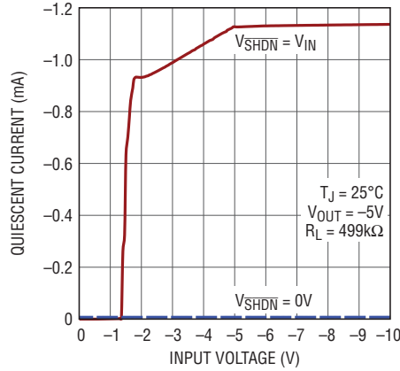
LT3015 Quiescent Current
