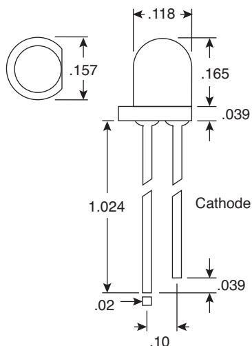
Dimensions (In.)
