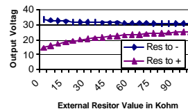
PM3024D15 Voltage Trim Adjusts the total voltage (+) out to (-) out
