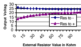
PM3024D12 Voltage Trim Adjusts the total voltage (+) out to (-) out
